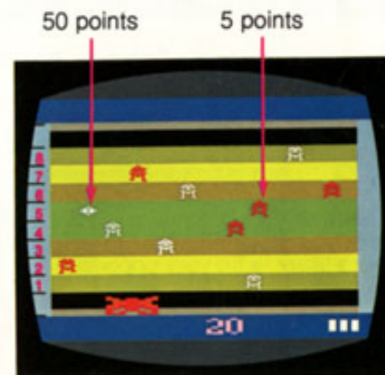
Figure 4 - Scoring System
