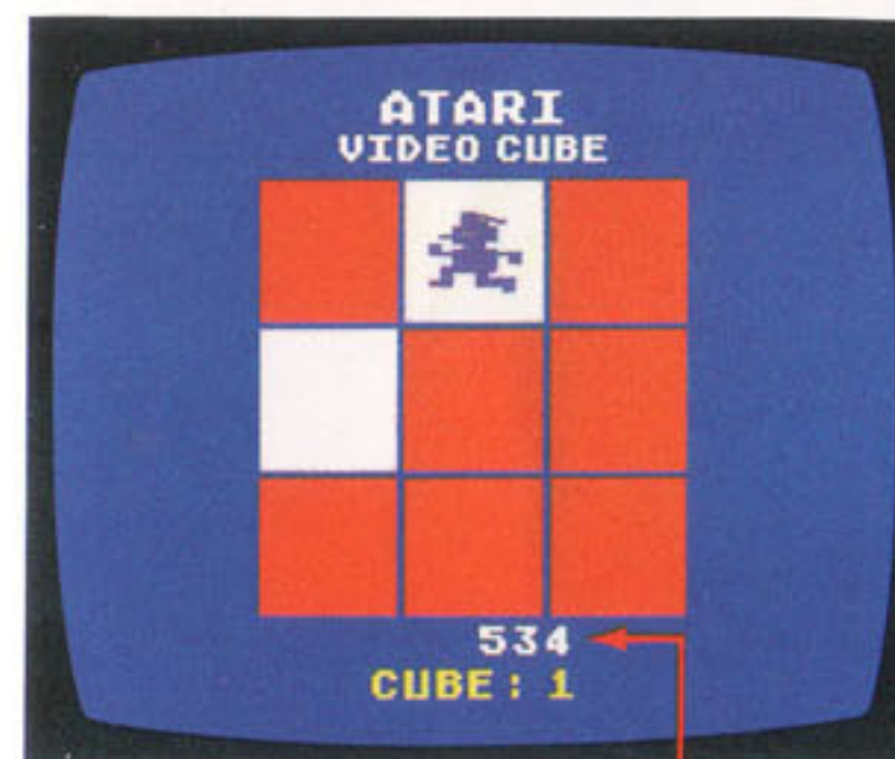
Score
