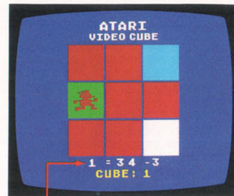
Score
