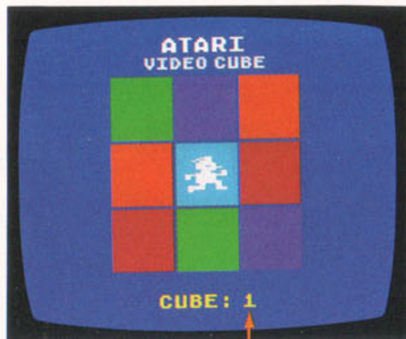
Cube Number
